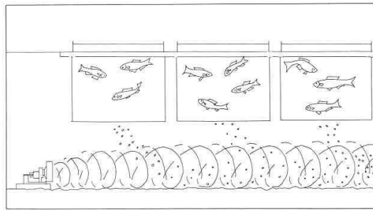
Fig. 2. Diagram of low-speed mixer installed on the bottom of a cage site to disperse wastes. (BEVERIDGE 1987)
