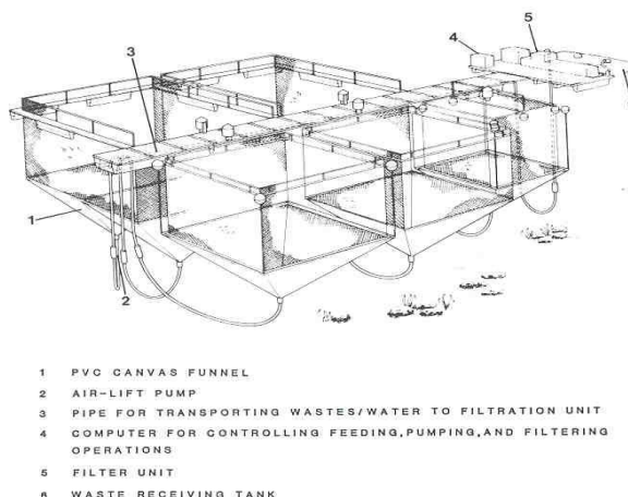
Fig. 3. Pilot computer controlled waste collection and uneaten feed retrieval system. (BEVERIDGE 1987)
