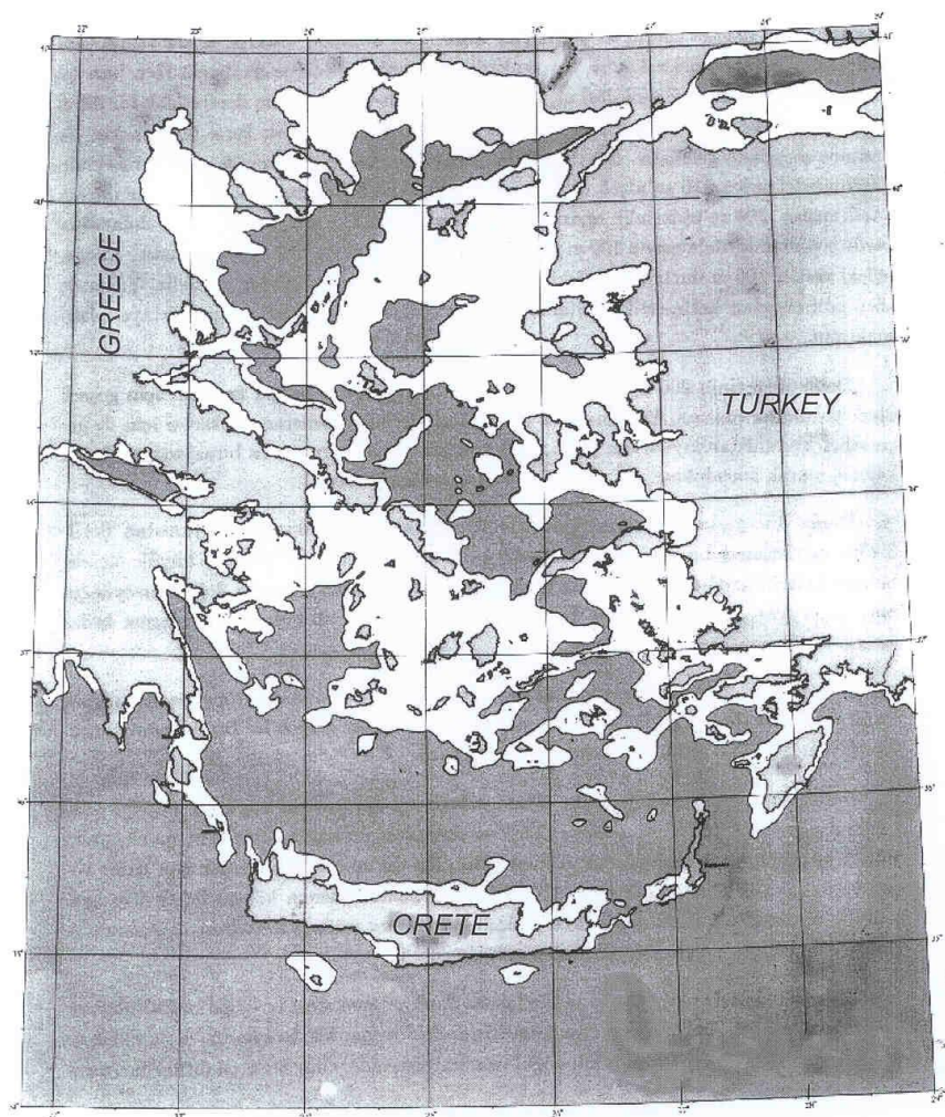
Figure 1. Configuration of land-masses in the Aegean sea area for a sea level 400 m lower than the present one. Blank areas at both sides of the narrow sea belt are emerged prolongations of the mainlands. Notice that emerged prolongation of the Turkish mainland extends near to Greek mainland in the central part of the Aegean, while the contrary is the case for the southern Aegean sea area.
